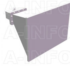
LB-510-15-C-7/16FSPO Standard Gain Horn Antenna 1.45-2.2GHz 15dB Gain 7/16(DIN) Female
